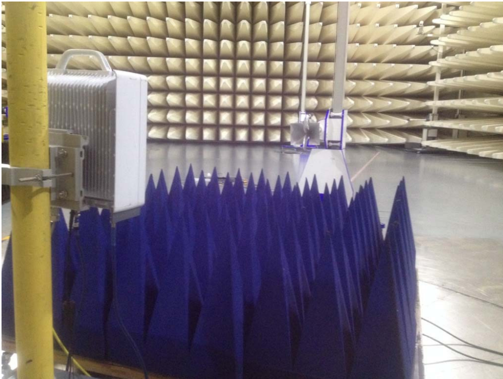
Radiated Emissions
