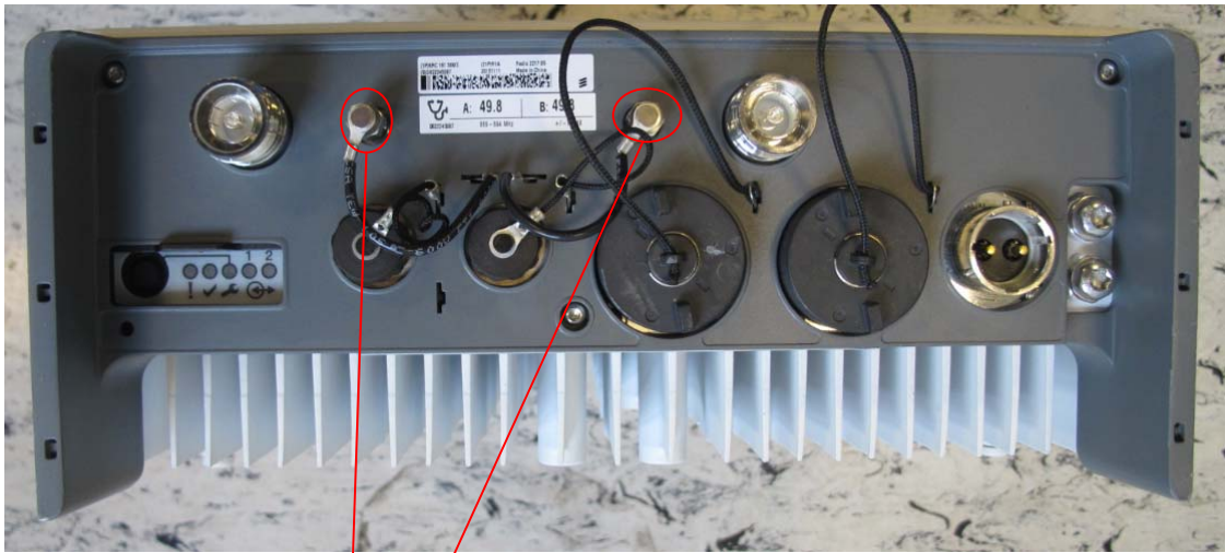
TX monitor ports
