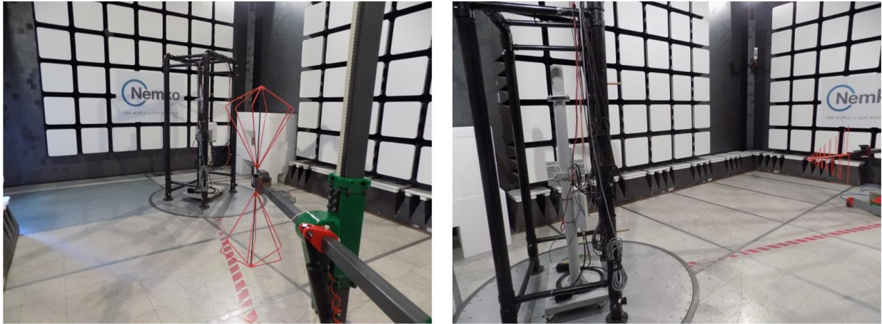
Figure 1: Radiated Test setup (30 to 1000MHz)
