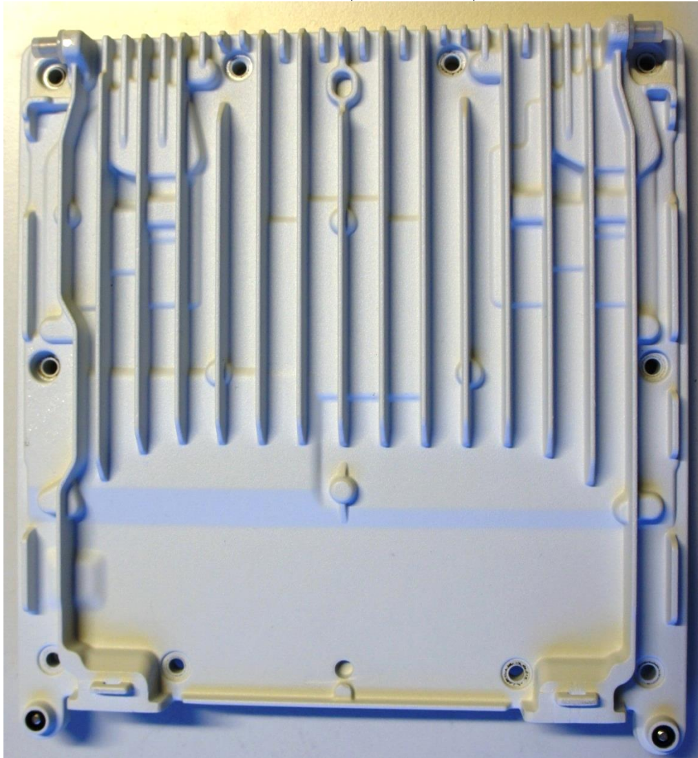
Rear side of Radio 2203 B66A, revision R1B, KRC 161 553/1
