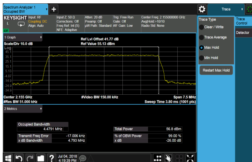
Port B , 16QAM 5.0M Channel Position M
