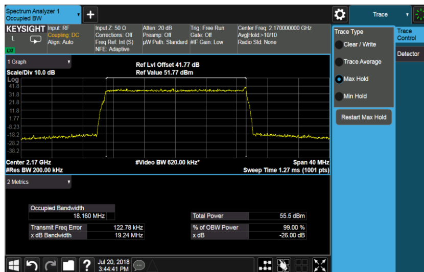
Port B , QPSK 20.0M Channel position T
