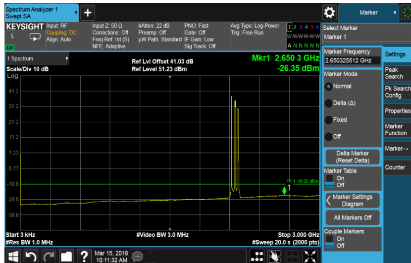
Port C, Channel Position M, LTE 15.0 MHz
