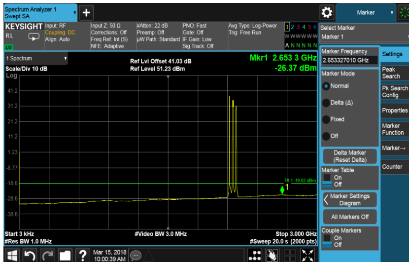
Port C, Channel Position M, LTE 10.0 MHz
