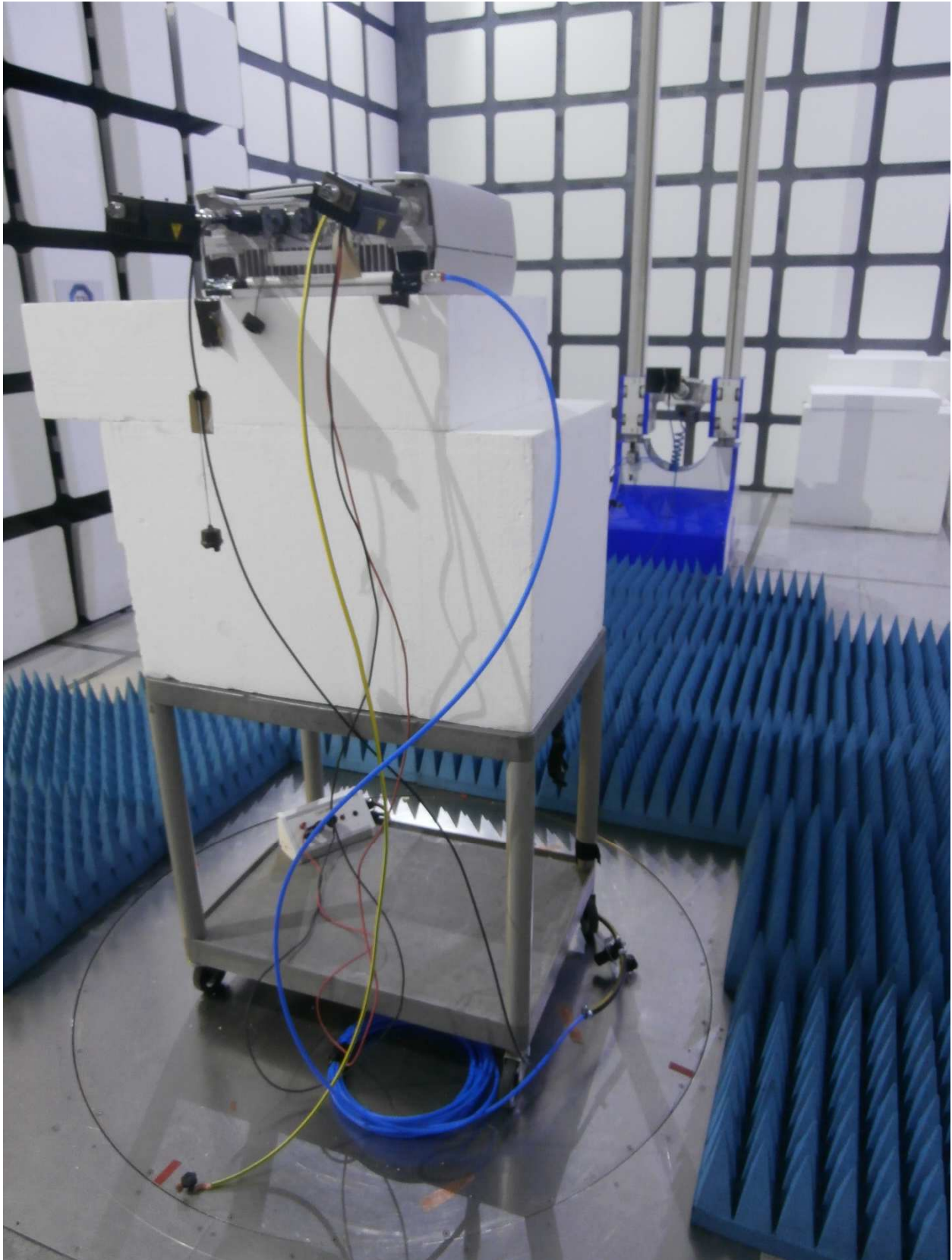
Radiated Emissions 1 GHz to 8 GHz
