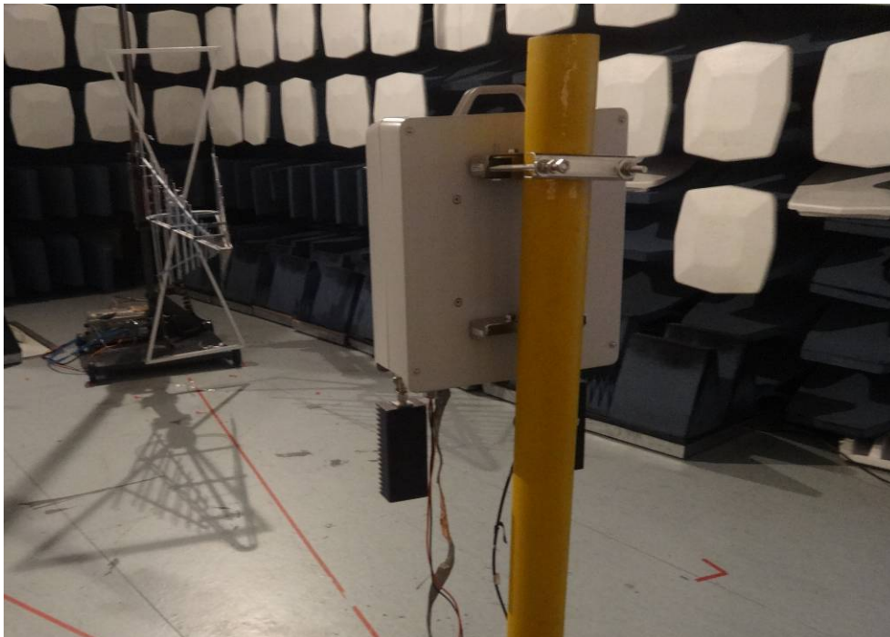
Radiated Emissions
