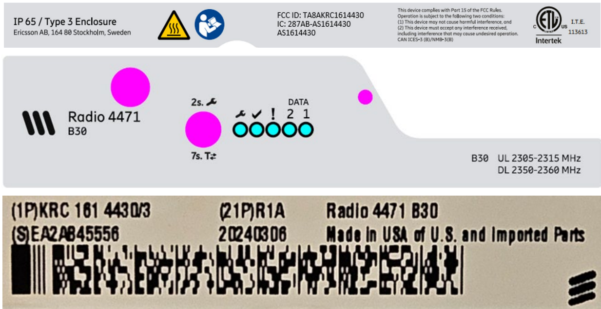
Figure 5: Radio 4471 B30 Product Labels
