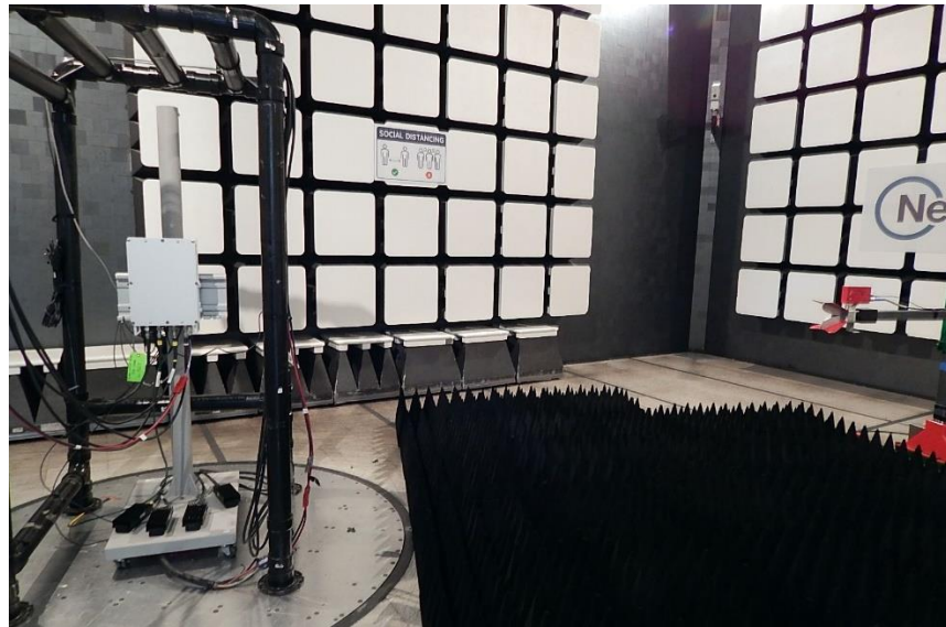
Figure Error! No text of specified style in document.-4: EUT Set-up photos for Cabinet Radiated Emissions above 1 GHz
