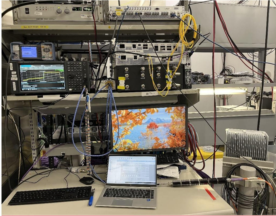
Figure Error! No text of specified style in document.-1: Set up photo for Radio Compliance Testing
