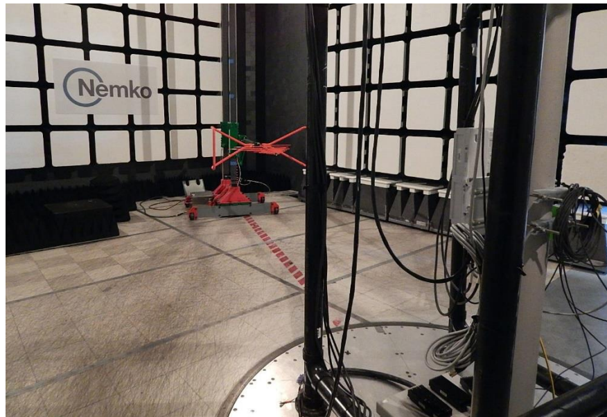
Figure Error! No text of specified style in document.-3: EUT Set-up photos for Cabinet Radiated Emissions below 1 GHz
