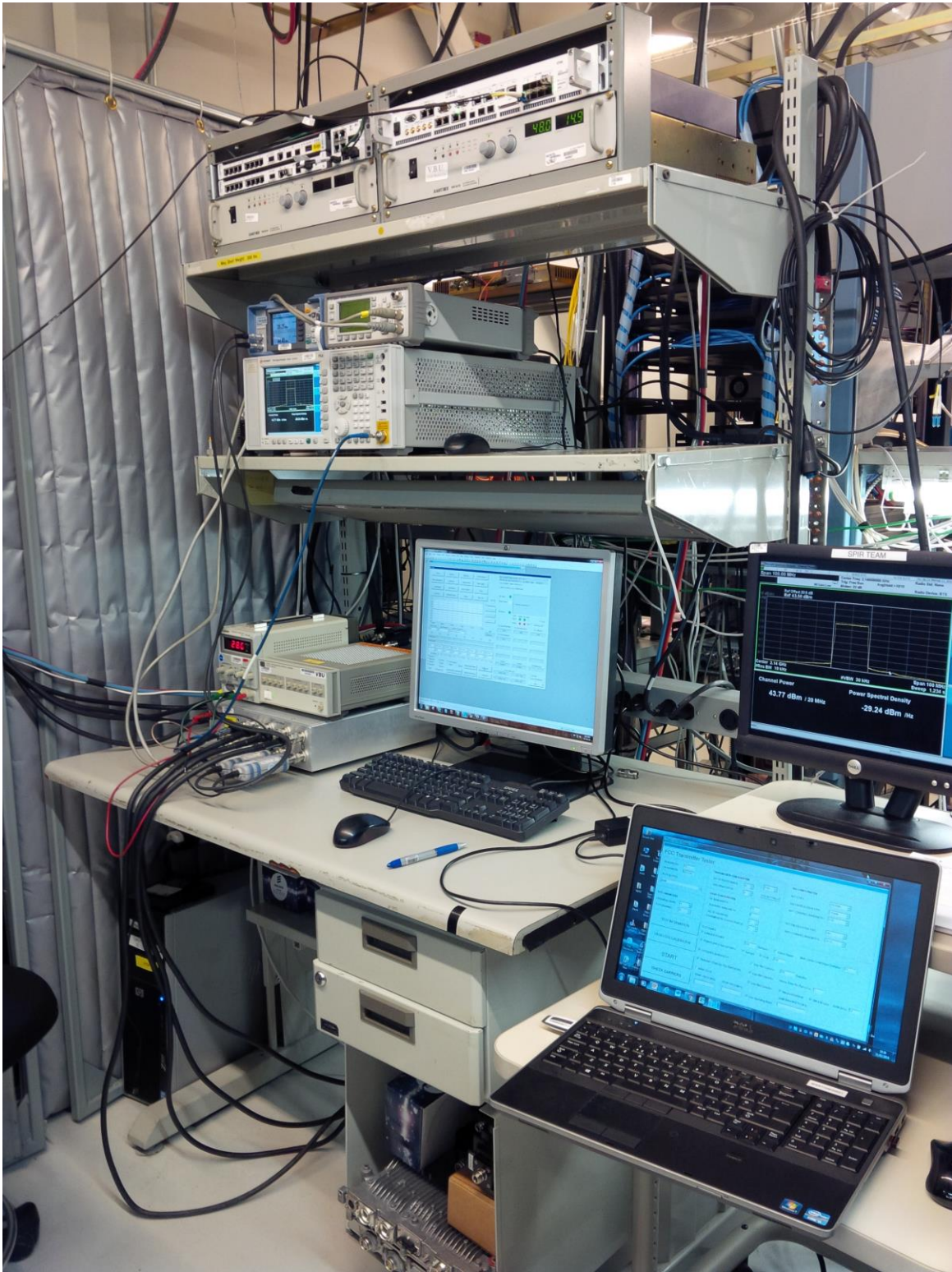
Figure 1: Test Equipment
