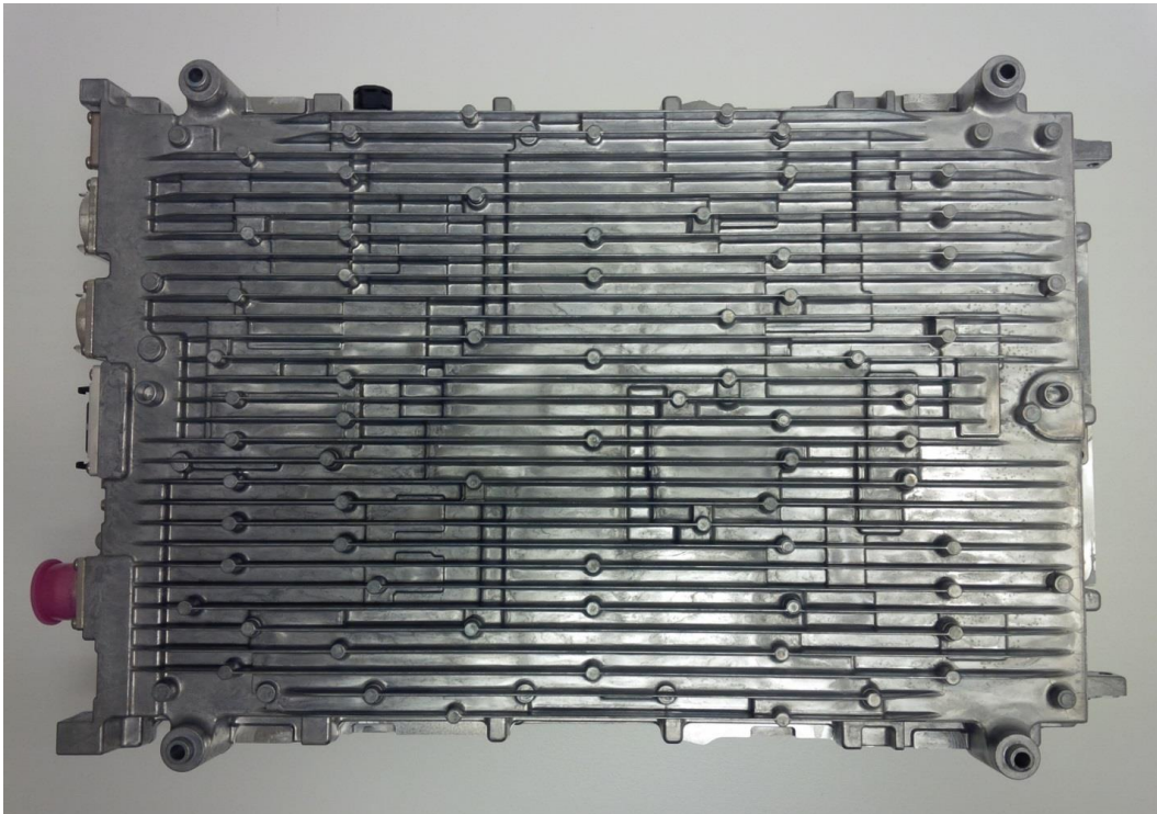
Figure 1: RRUS 32A B2 Bottom View
