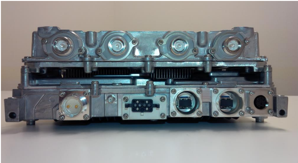
Figure 4: RRUS 32A B2 Front View
