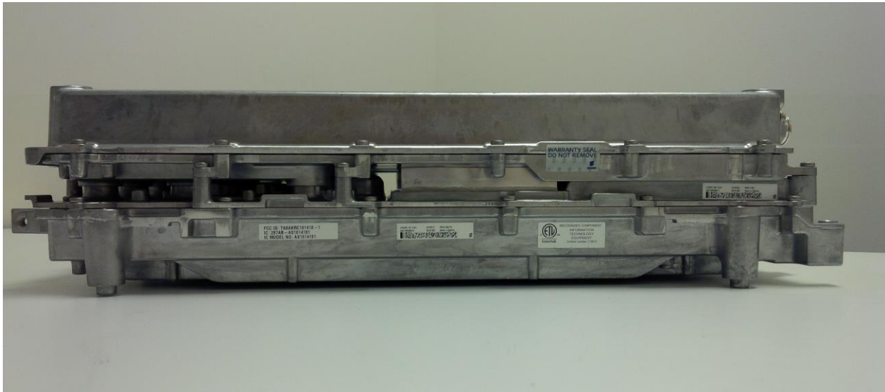
Figure 5: RRUS 32A B2 Left Side View
