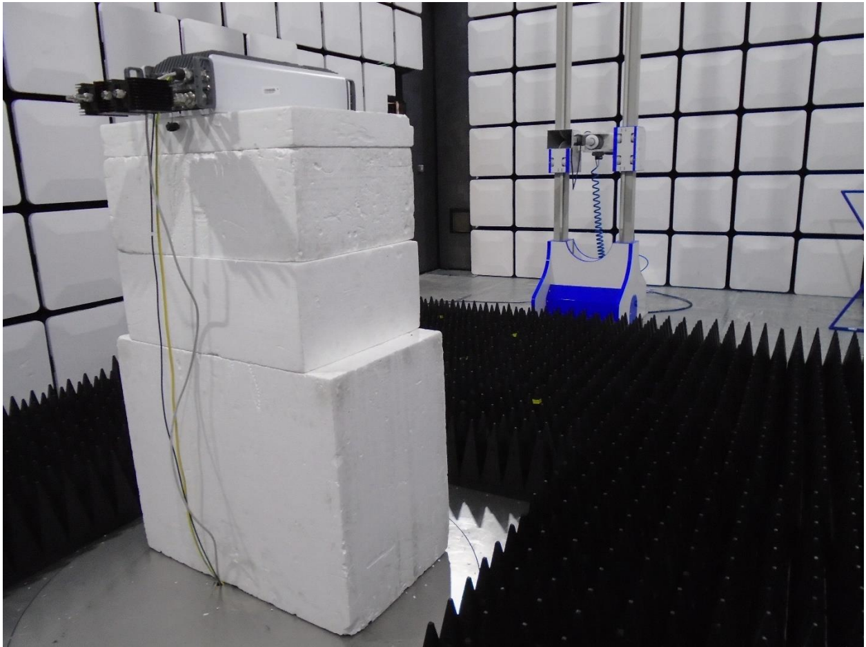
Radiated 1GHz – 18GHz Testing
