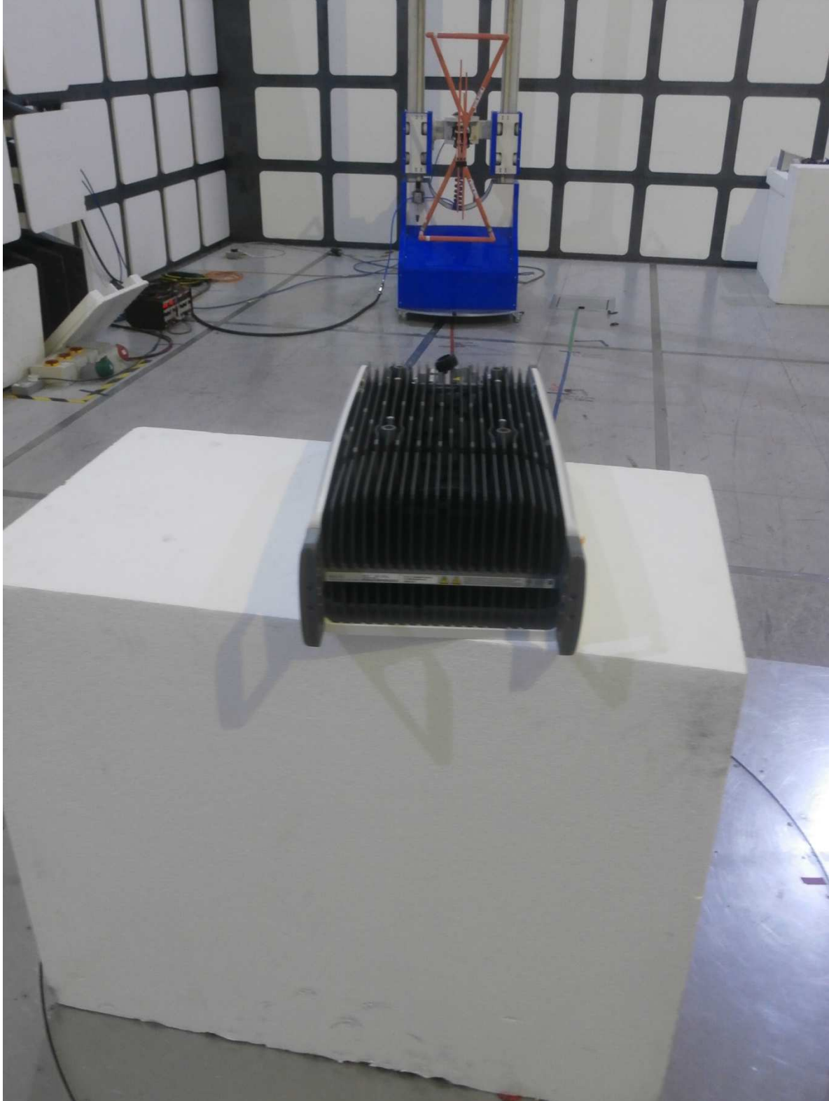
Radiated Emissions 30 MHz to 1 GHz
