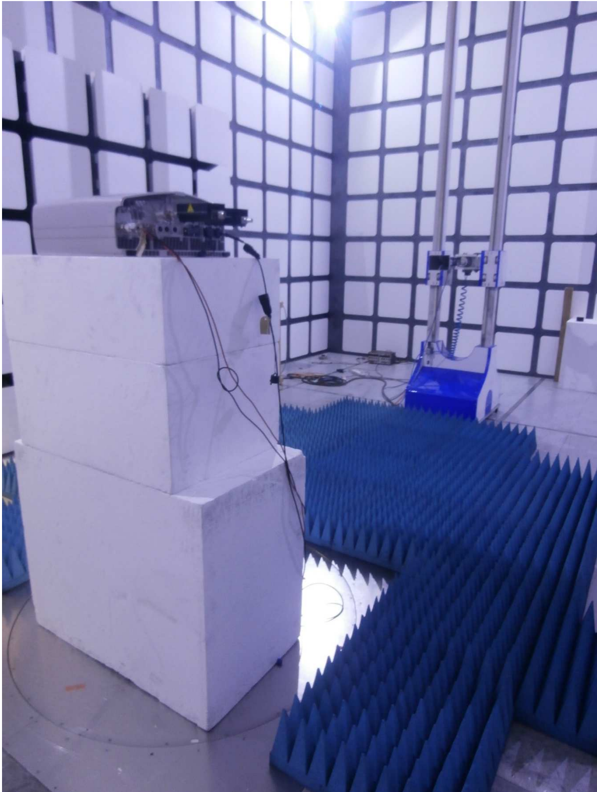
Radiated Emissions 1 GHz to 8 GHz
