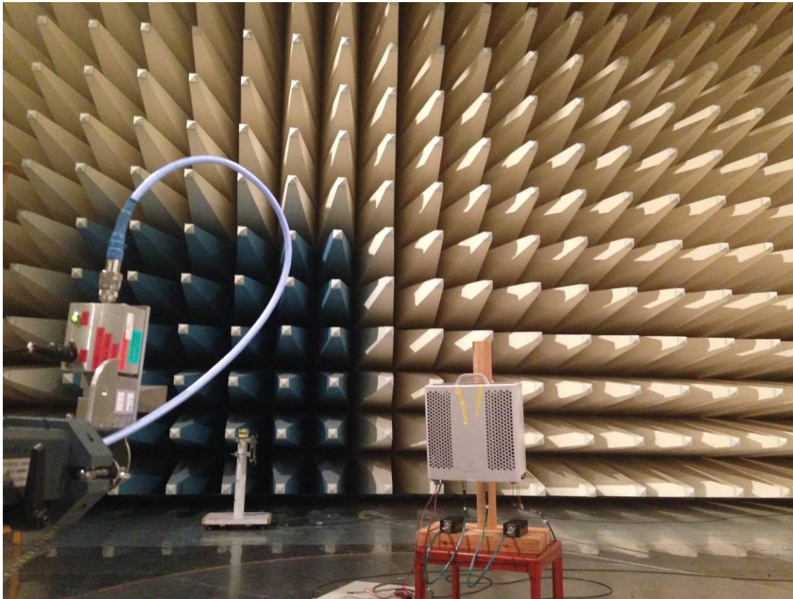
Radiated Emissions
