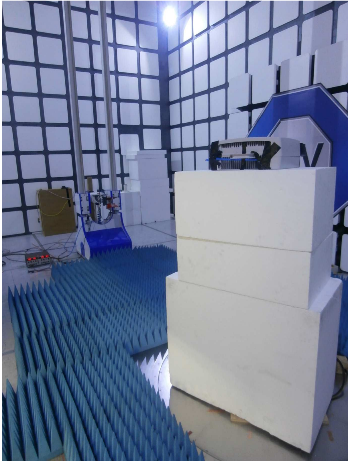
Radiated Emissions 8 GHz to 18 GHz
