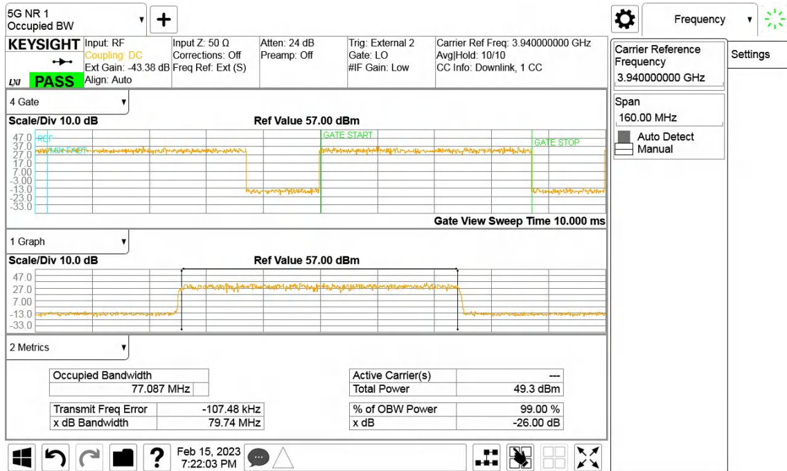
QPSK, 80MHz, Channel position T, B77D
