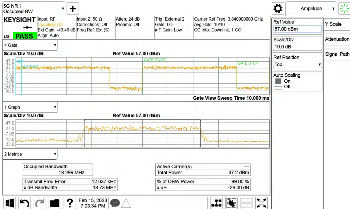
QPSK, 20MHz, Channel position M, B77D
