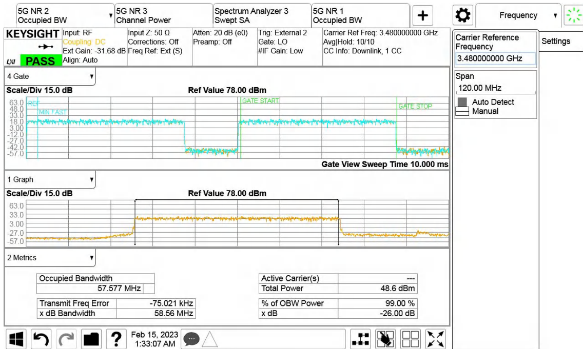
QPSK, 60MHz, Channel position B, B77G
