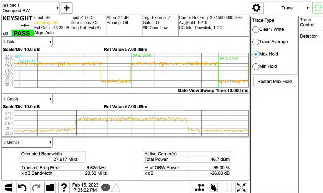
QPSK, 30MHz, Channel position B, B77D
