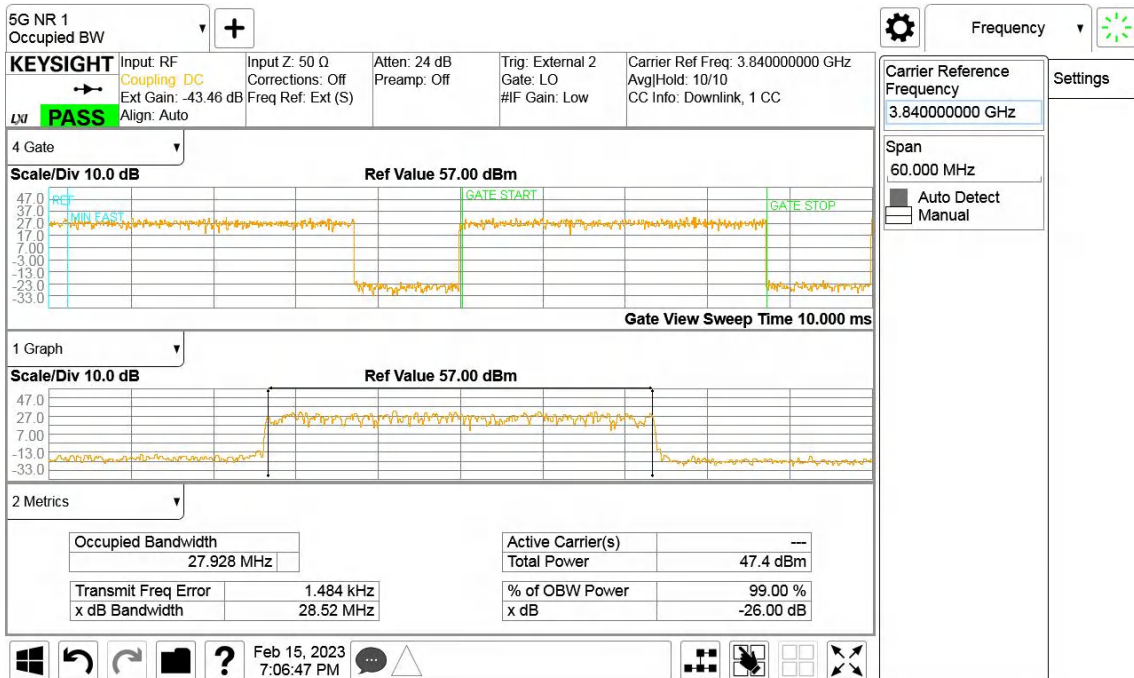
QPSK, 30MHz, Channel position M, B77D
