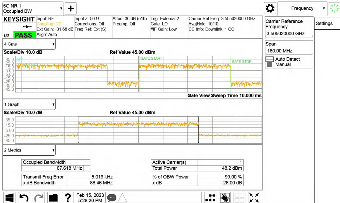
QPSK, 90MHz, Channel position T, B77G
