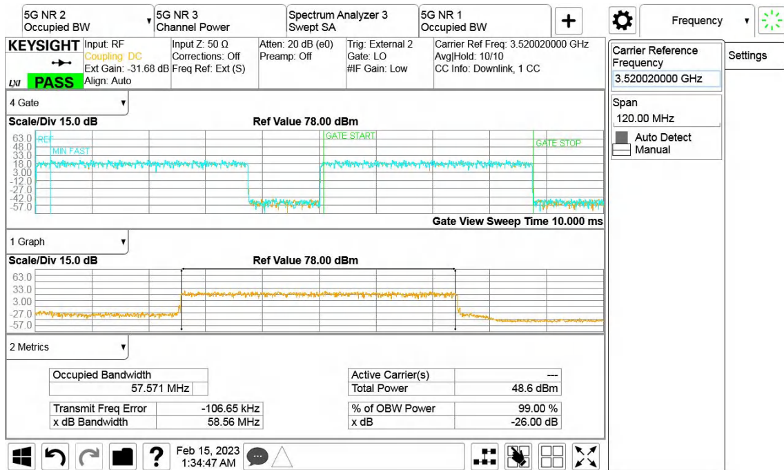
QPSK, 60MHz, Channel position T, B77G
