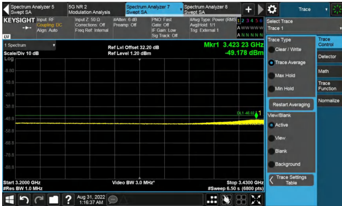
Channel Position M, 3200MHz to 3430MHz
