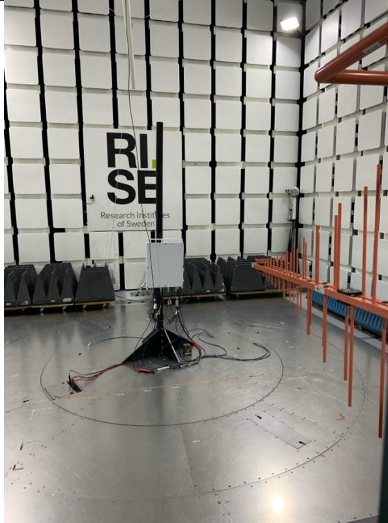
Test setup 30-1000 MHz:
