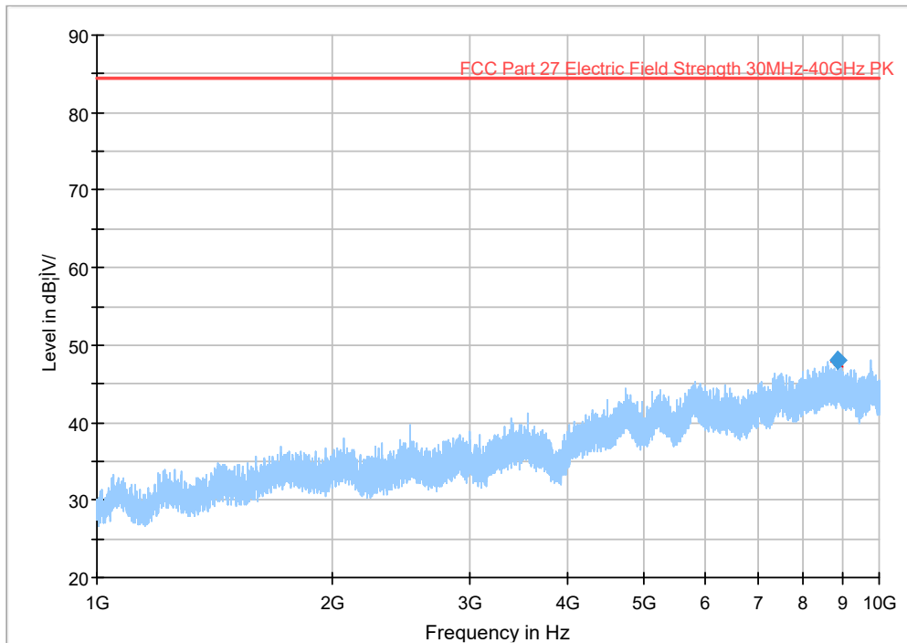
1-10GHz, Vertical
