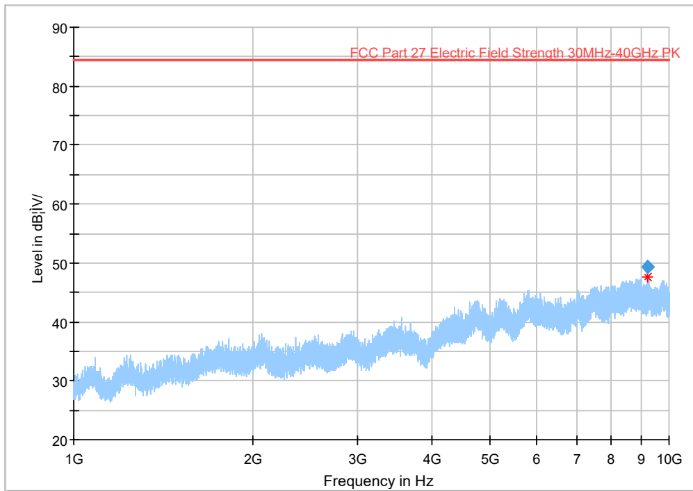
1-10GHz, Vertical
