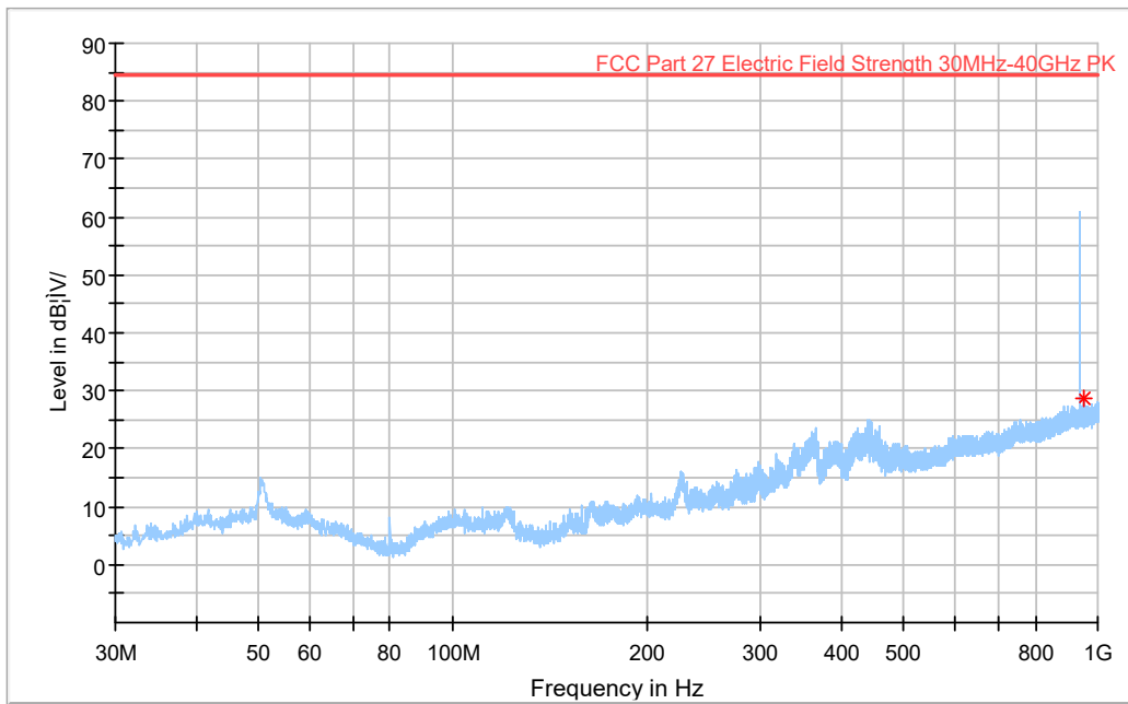
30-1000MHz, Vertical
