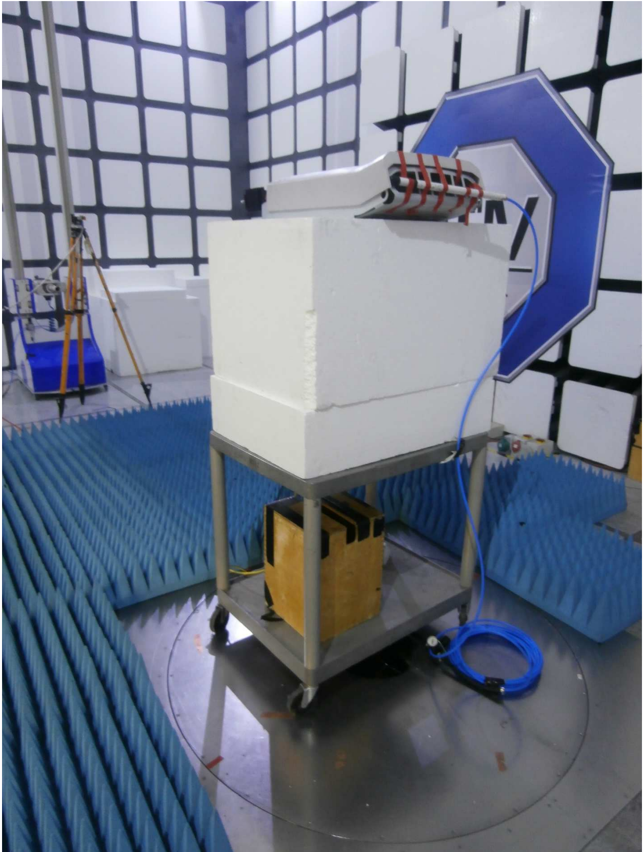
Radiated Emissions 18 GHz to 25 GHz
