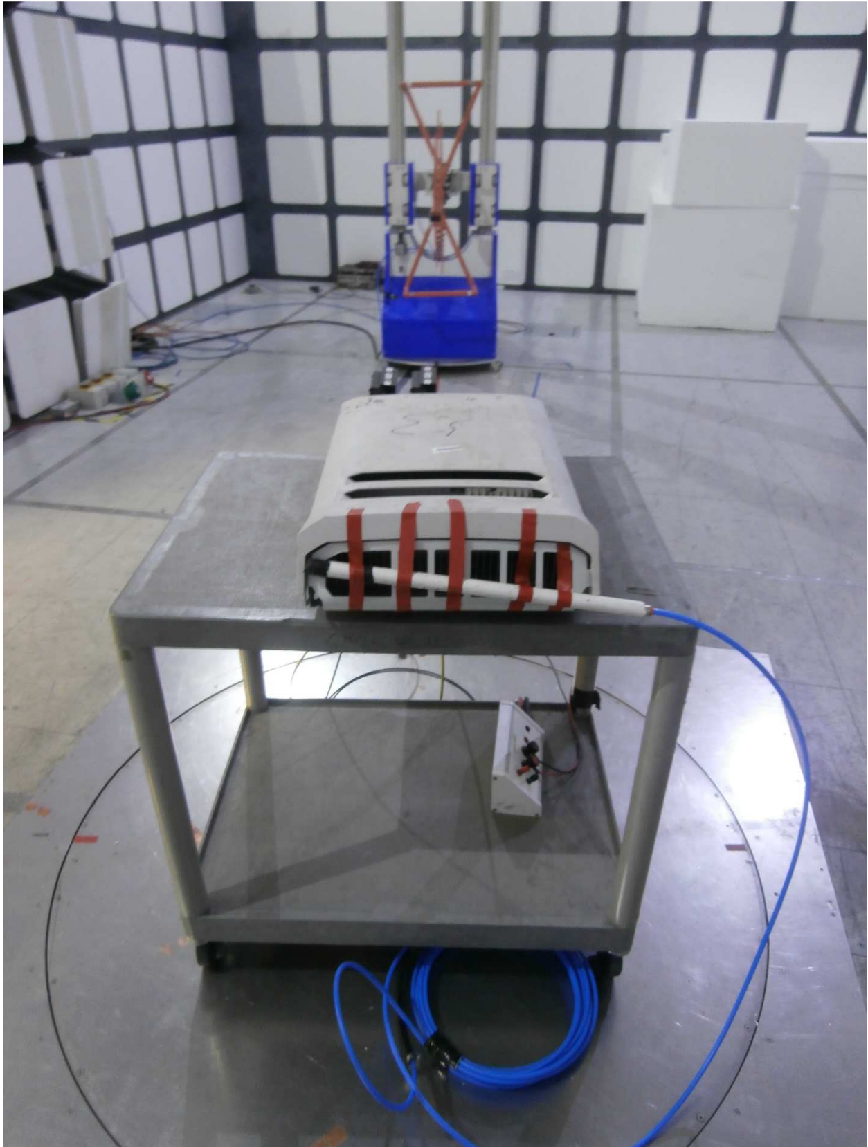
Radiated Emissions 30 MHz to 1 GHz
