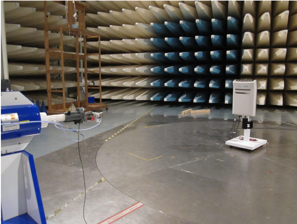
Radiated Emissions
