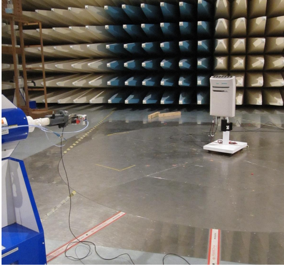
Radiated Emissions
