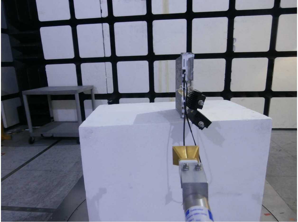
Radiated Emissions 18 GHz to 25 GHz
