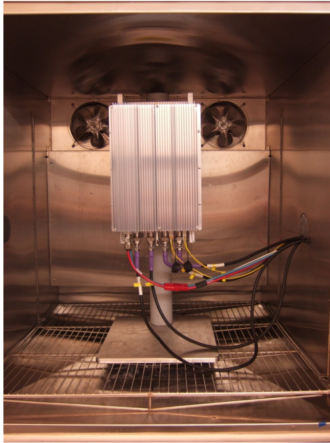
Lab Testing – Base Station in Temperature Chamber
