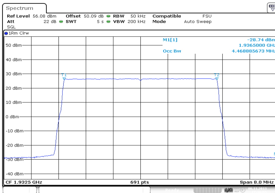
Measurement 99 % Occupied Bandwidth - Channel Position B - Carrier Bandwidth 5.0 MHz
