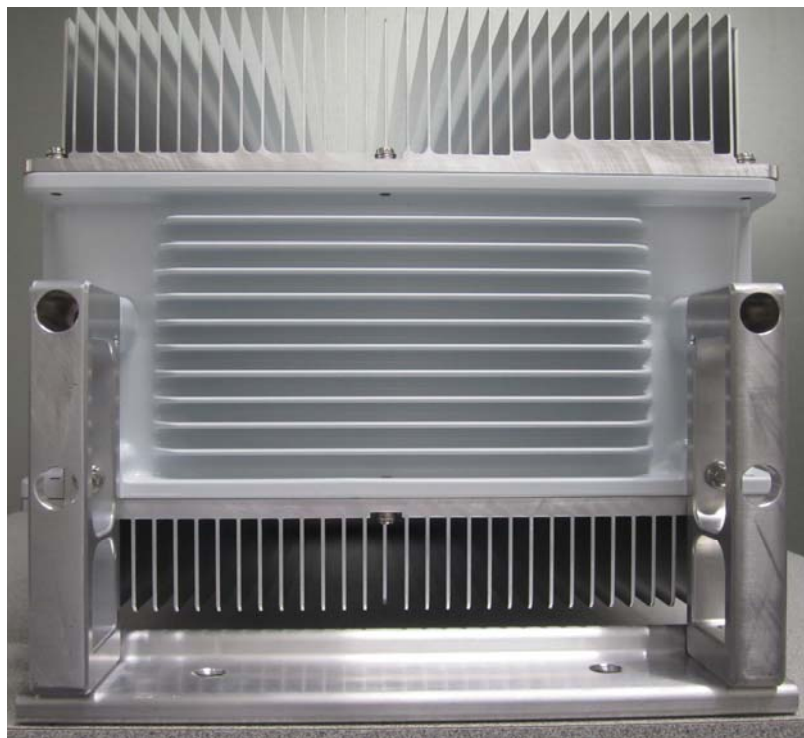
Figure 2: RRUS 31 Top View
