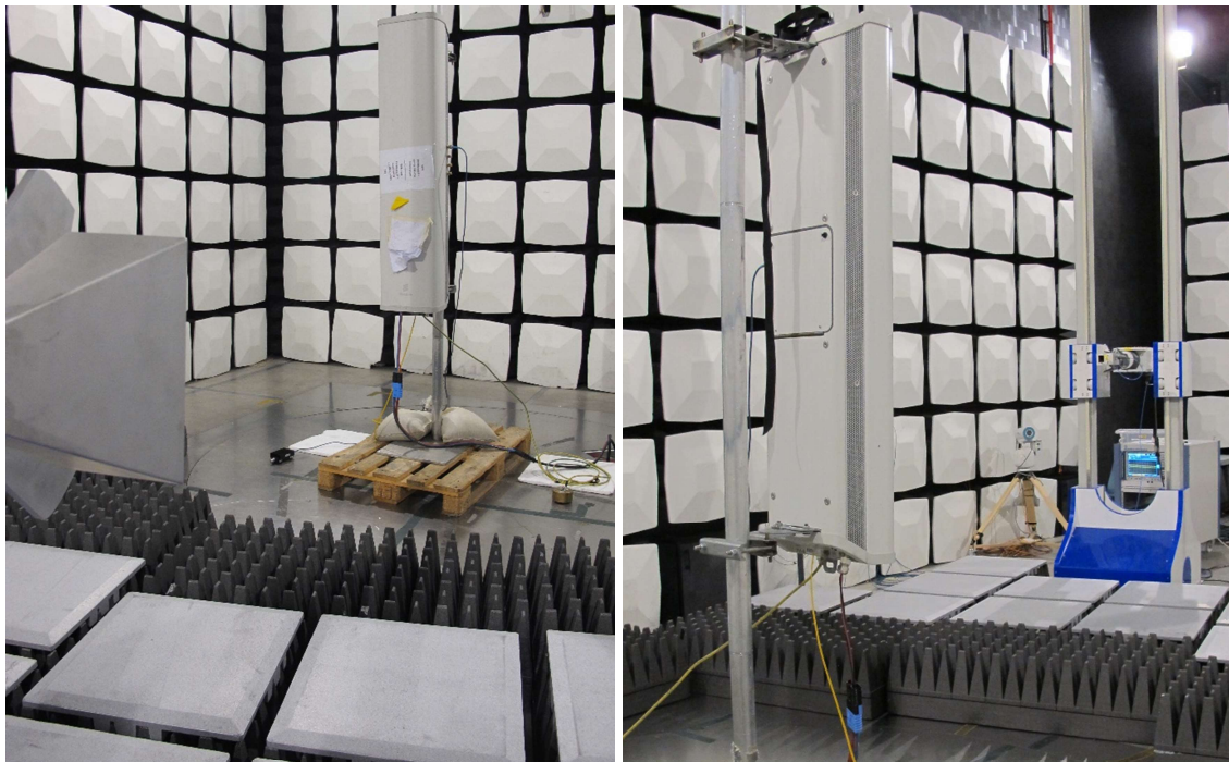
Photos of the test set up
