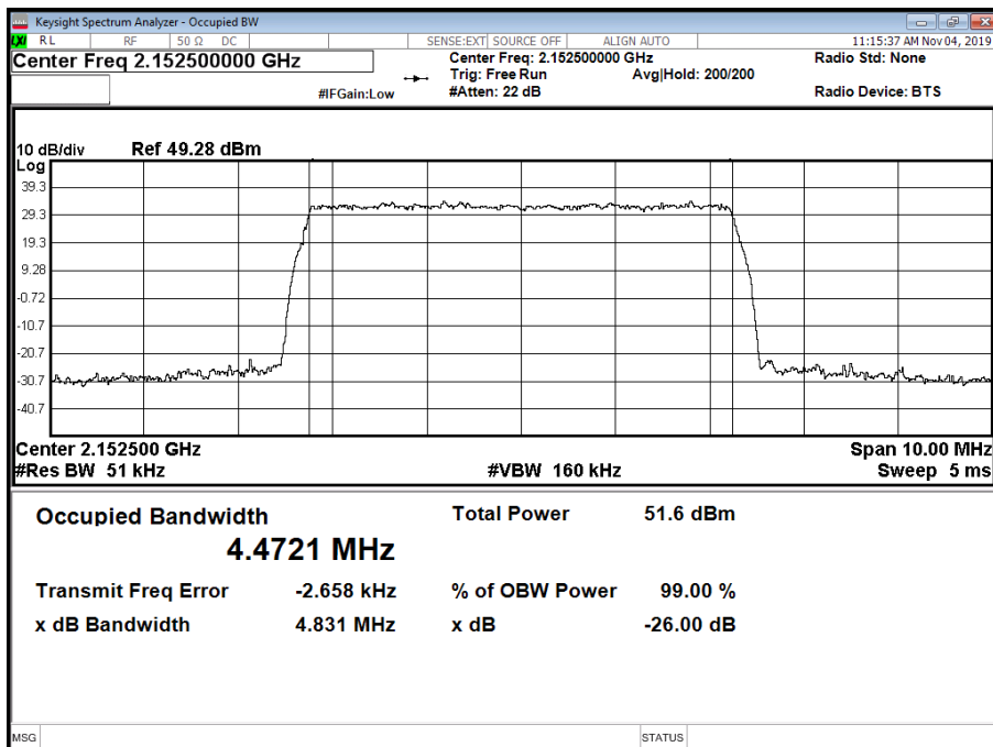
Antenna A - NR Modulation QPSK - NR Carrier Bandwidth 5.0 MHz 15 kHz SCS - Channel Position T
