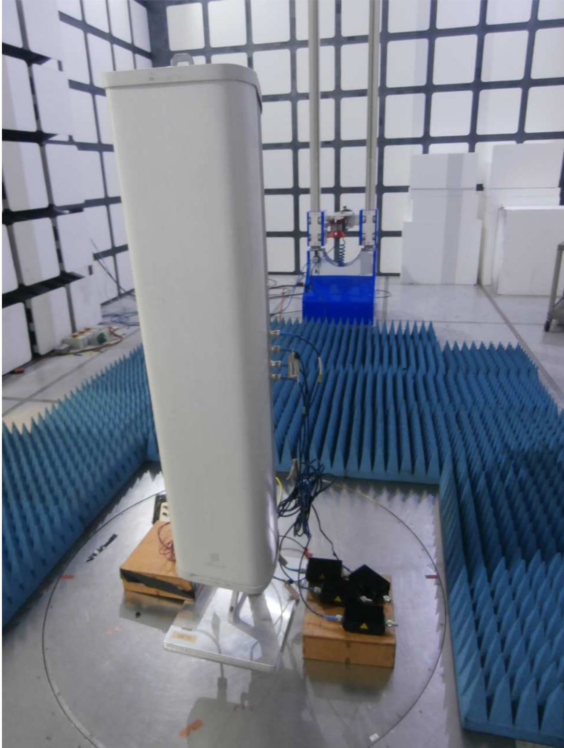
Radiated Emissions 8 GHz to 18 GHz
