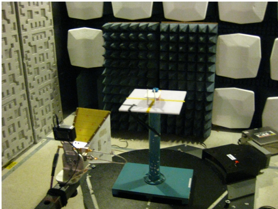
EUT on Test Pedestal
