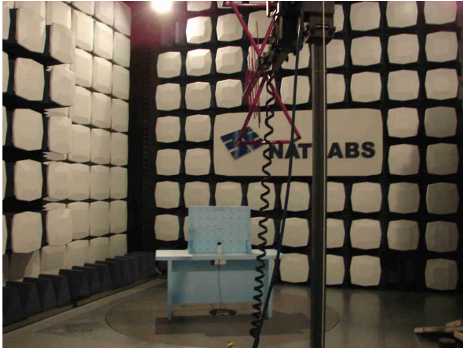
Picture 1: Spurious emission measurement and Radiated emission test setup
