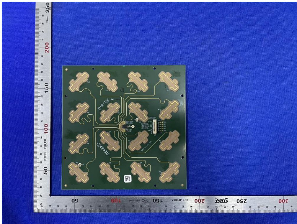
(CC2642R1F) BLE2 Antenna
