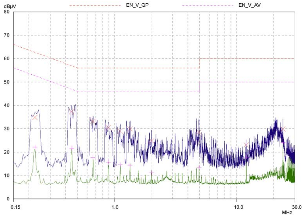
Figure 10. Plot of the Conducted Emissions Line – PE
