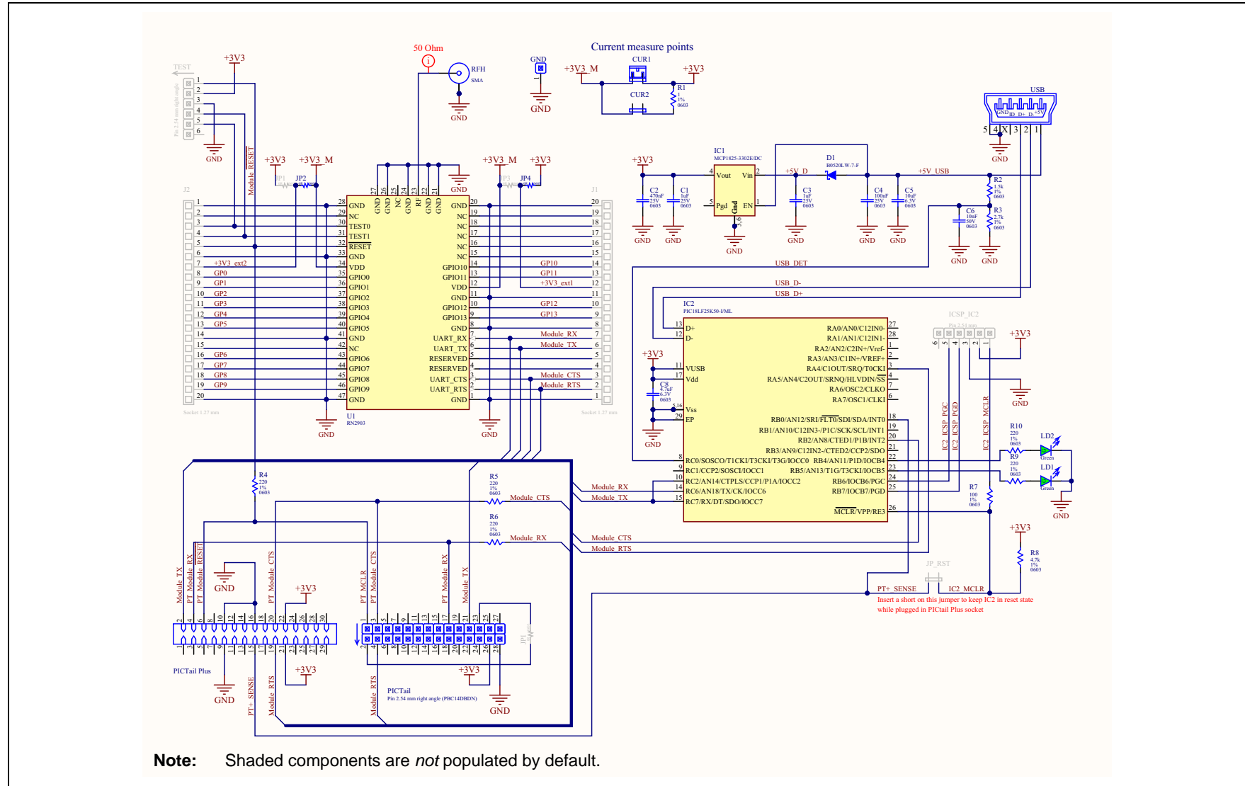
FIGURE 5-6: PICTAIL™/PICTAIL PLUS DAUGHTER BOARD SCHEMATIC
