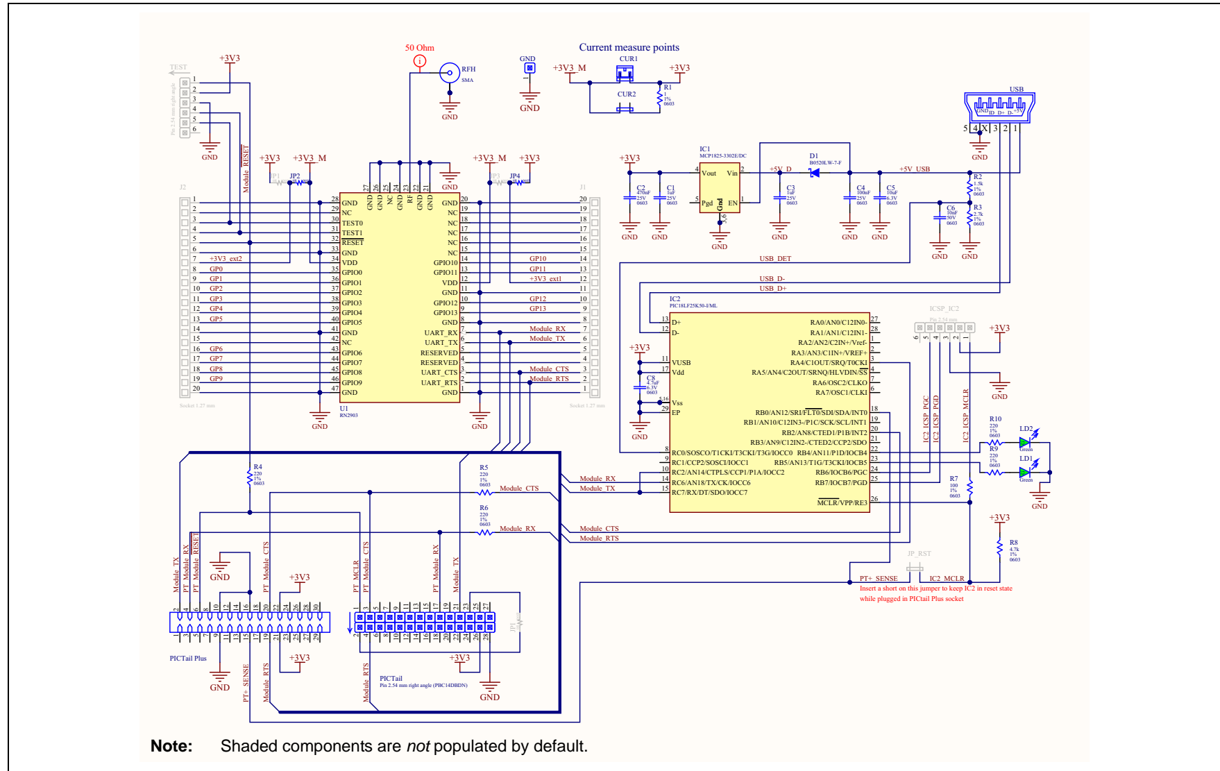
FIGURE 5-2: PICTAIL™/PICTAIL PLUS DAUGHTER BOARD SCHEMATIC
