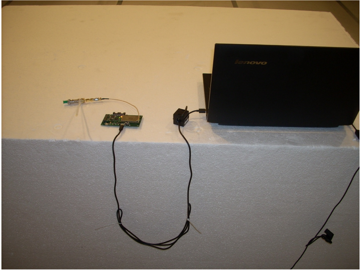
Radiated Emissions below 1 GHz – Front View
