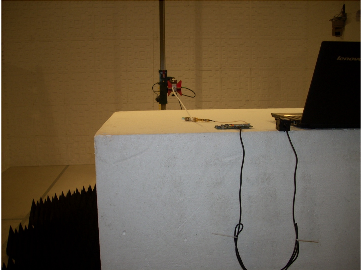
Radiated Emissions above 1 GHz – rear View
