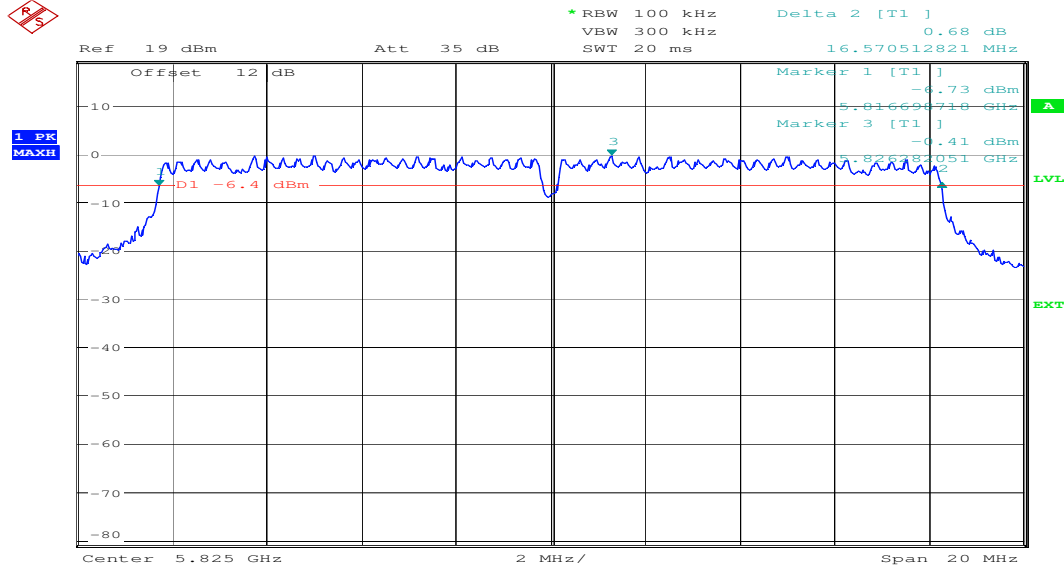
Plot 3: 6 dB-Bandwidth (5825 MHz)
