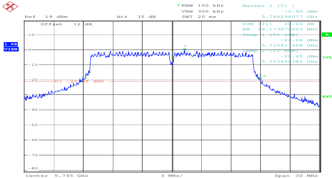
Plot 4: 20 dB-Bandwidth (5745 MHz)
