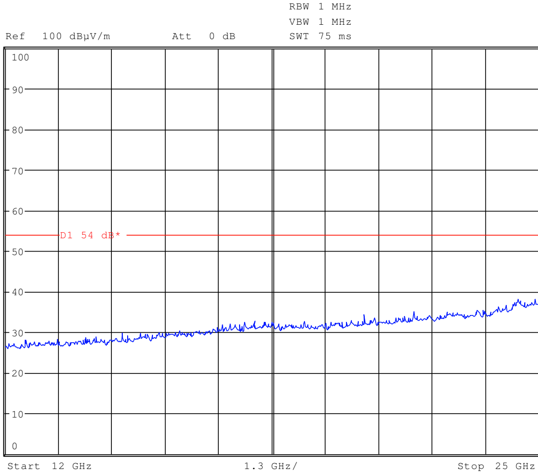
Plot 4: 12 – 25 GHz horizontal / vertical (valid for all three channels)
