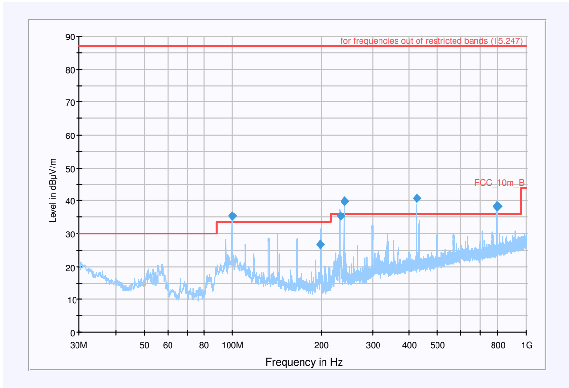
Plot 7: 0.03 - 1 GHz vertical / horizontal (middle channel)
