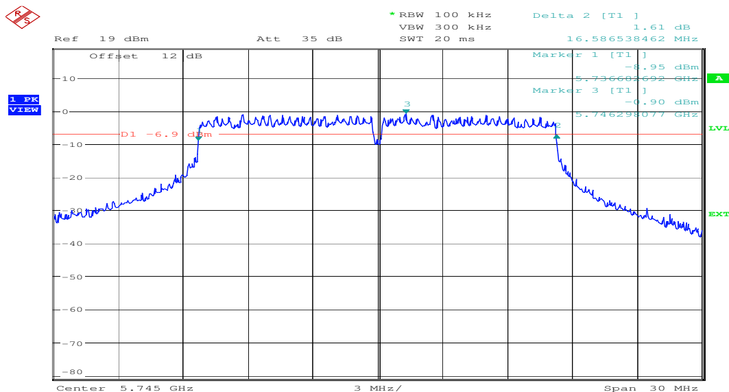
Plot 1: 6 dB-Bandwidth (5745 MHz)
