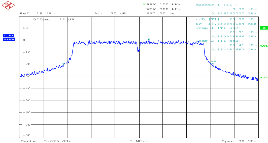
Plot 6: 20 dB-Bandwidth (5825 MHz)
