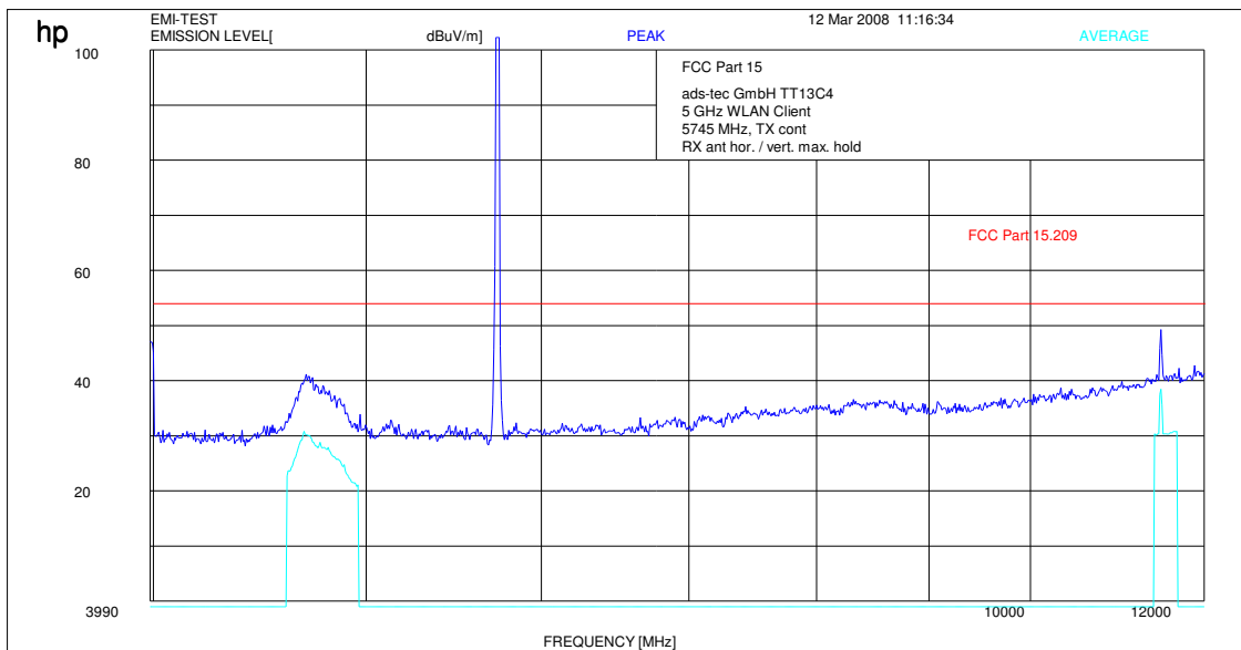
Plot 3: 4-12 GHz (lowest channel)
