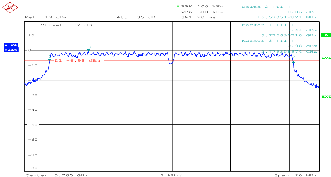
Plot 2: 6 dB-Bandwidth (5785MHz)
