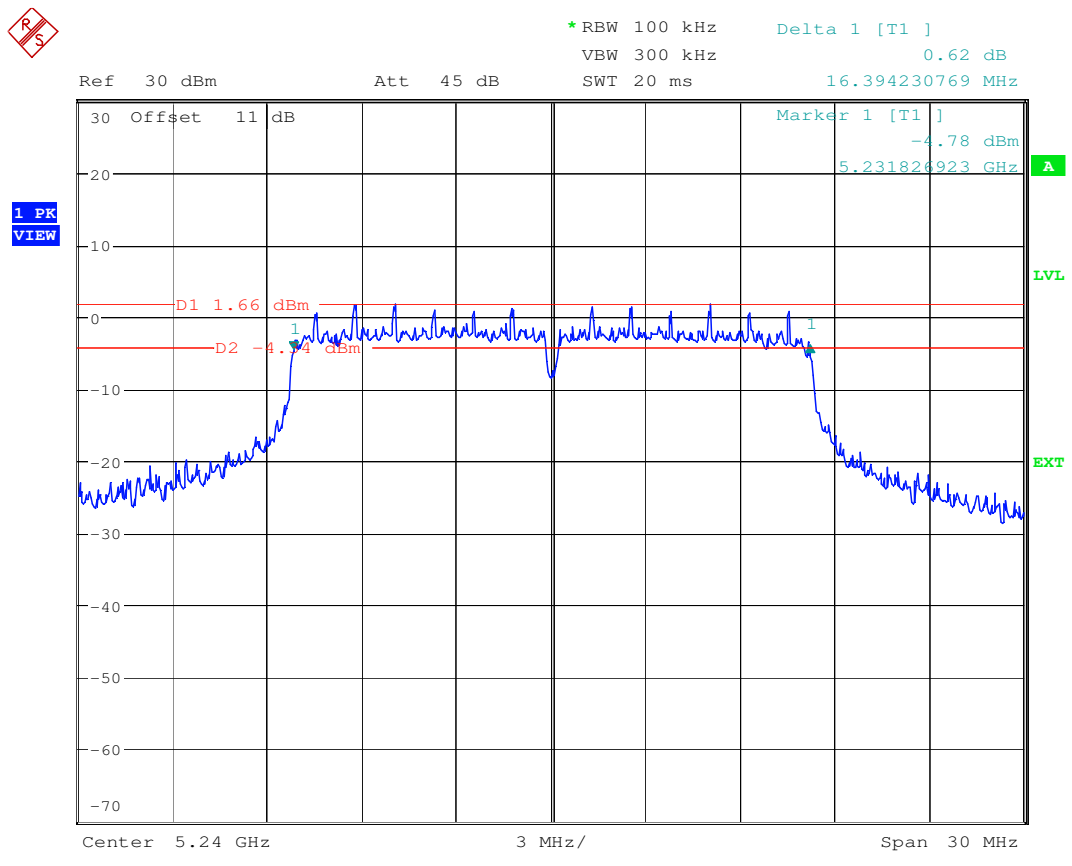
Plot 7: 5240 MHz 6 dB BW
