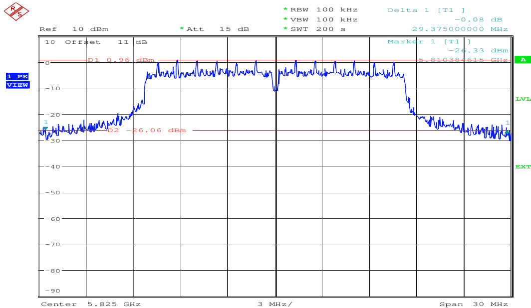
Plot 9: 26 dB-Bandwidth (5825 MHz)
