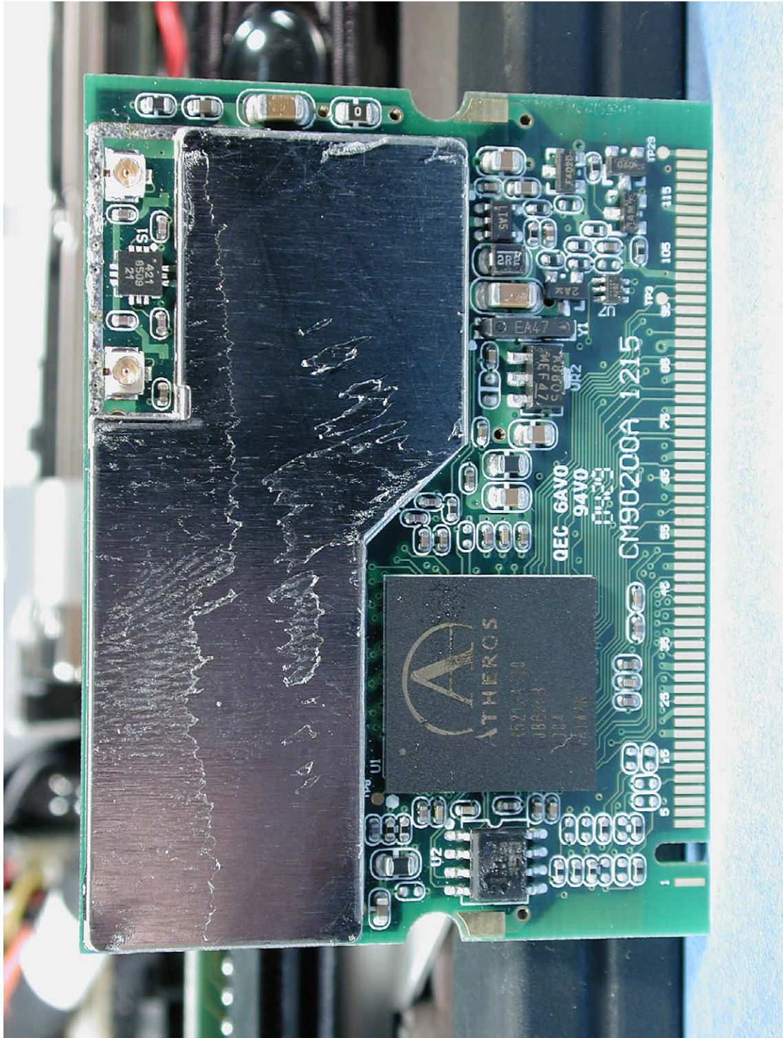
Photograph 3: WLAN card PCB (top side)
