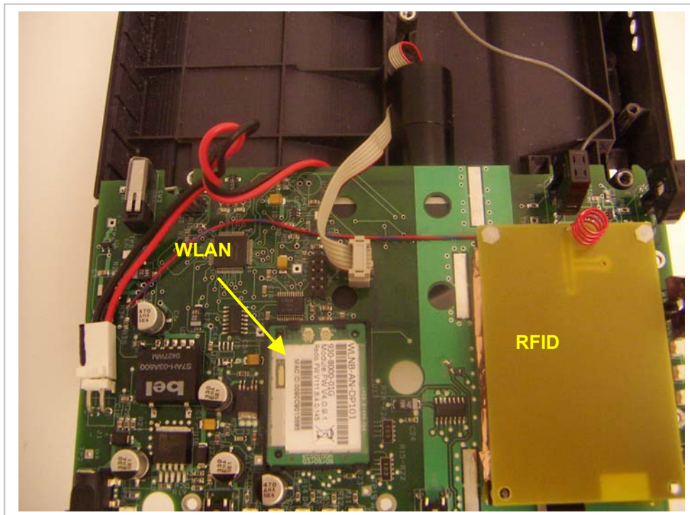
RFID Location
