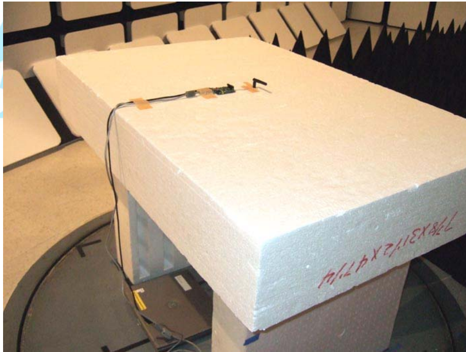
EUT Setup [Dipole antenna]: BG1
