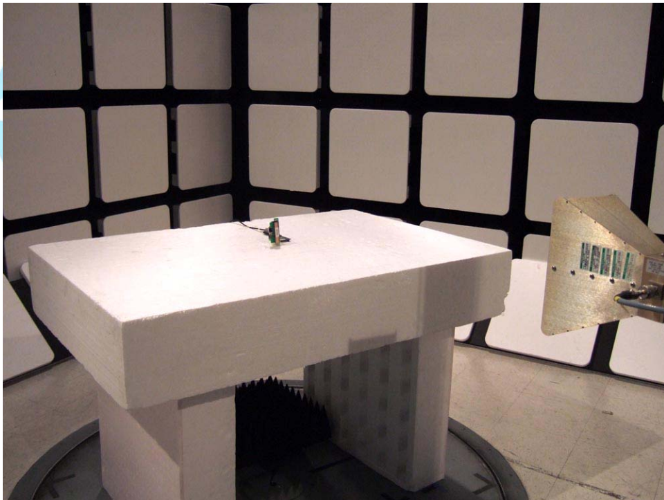
Test Configuration 2: 960 MHz – 40 GHz, BG1 and BG3 worst case [XZ]
