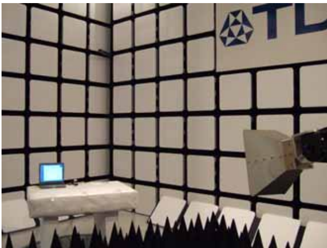
Test Configuration 2: 960 MHz to 40 GHz
