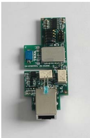
Bluetooth and Serial board top
