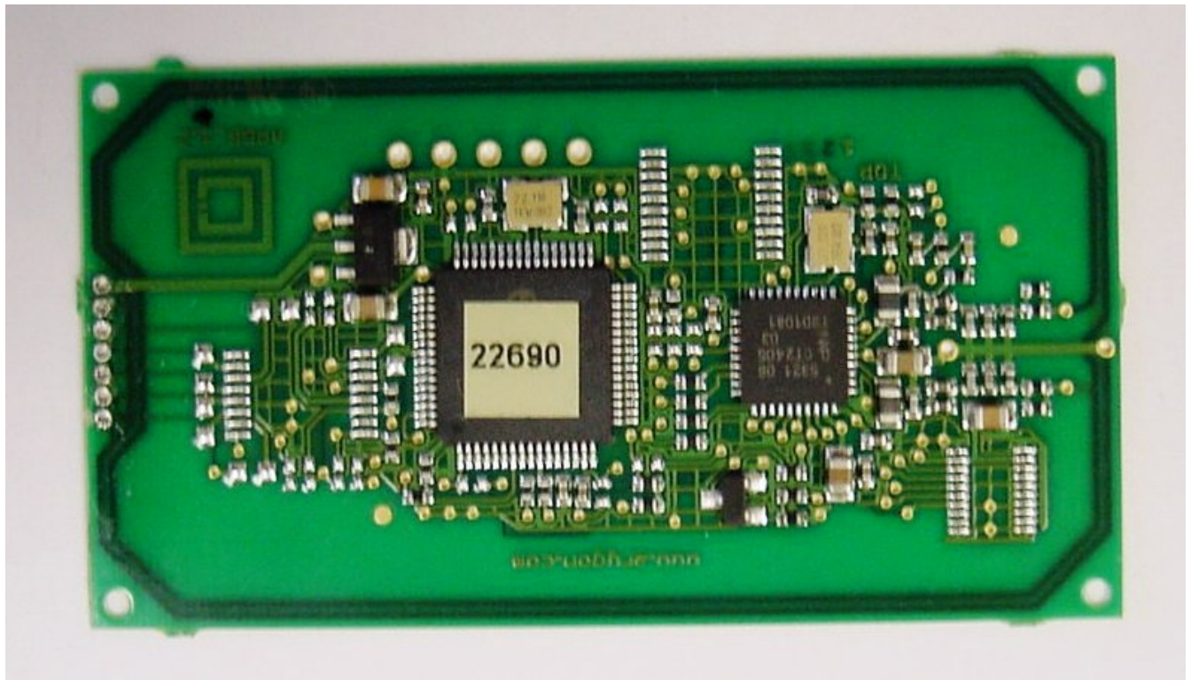
Photo Description: RF Board – Side 1:
