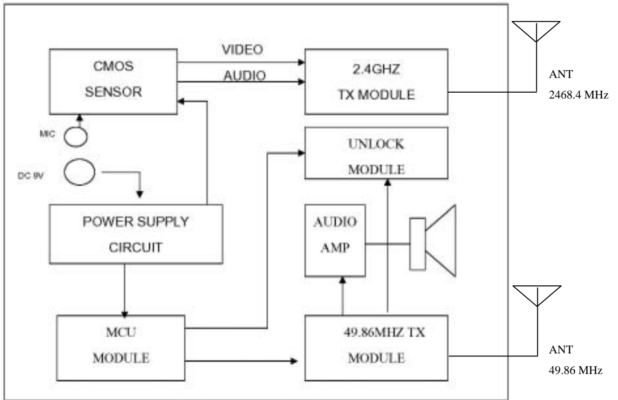
SB-101BWL BLOCK DIAGRAM
